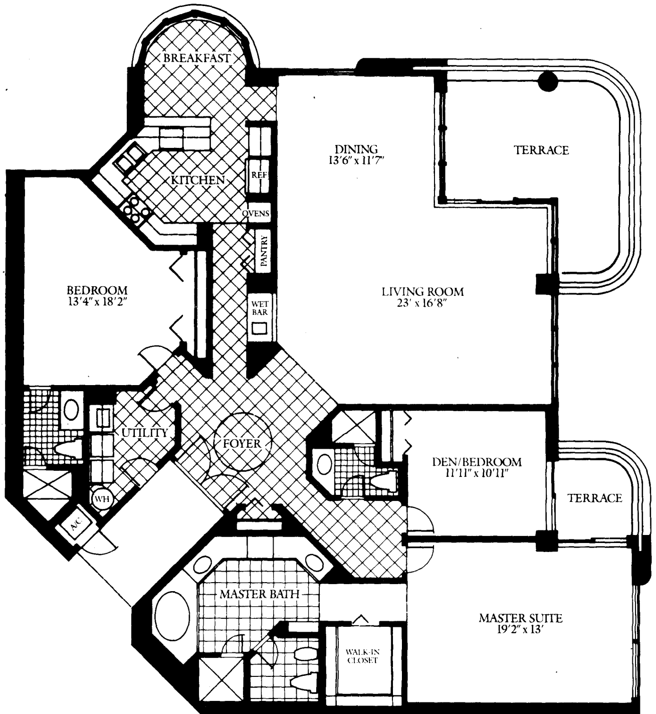
RESIDENCE TYPE "D" FLOOR PLAN (2327 SQ. FT.)
